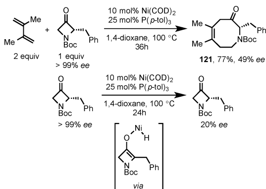
Scheme 39. Ni/P( p -tol) 3 -Catalyzed Cycloaddition of Diene with Chiral 2-Substituted Azetidinone and Loss of Enantioselectivity of Chiral Azetidinone
