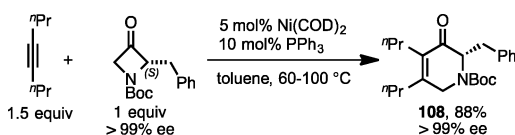
Scheme 34. Ni/PPh 3 -Catalyzed Cycloaddition of 4-Octyne and Chiral 2-Substituted Azetidinone
