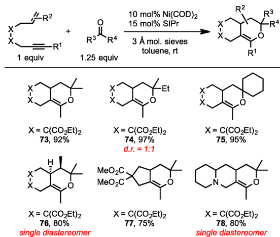
Scheme 27. Ni/SIPr-Catalyzed Cycloaddition of Enynes and Ketones
