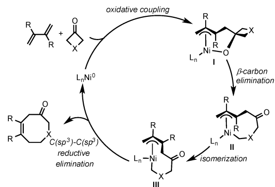
Scheme 40. Proposed Mechanism of Ni/P( p -tol) 3 -Catalyzed Cycloaddition of 1,3-Dienes with 3-Azetidinones and 3-Oxetanones
