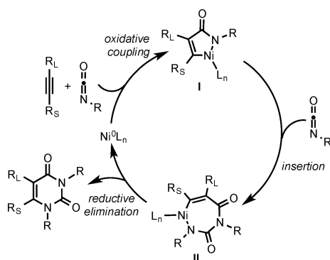
Scheme 10. Proposed Mechanism for the Synthesis of Pyrimidine-Diones
