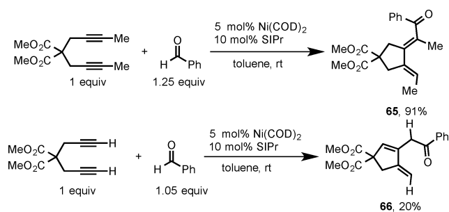
Scheme 23. Ni/SIPr-Catalyzed Cycloaddition of Internal 2,7-Diyne and Terminal 1,6-Diyne with Benzaldehyde
