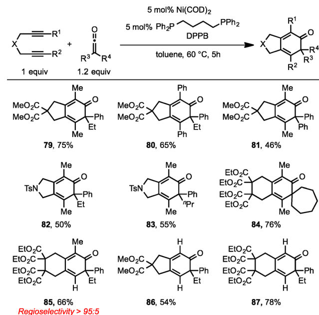
Scheme 29. Ni/DPPB-Catalyzed Cycloaddition of Diynes and Ketenes
