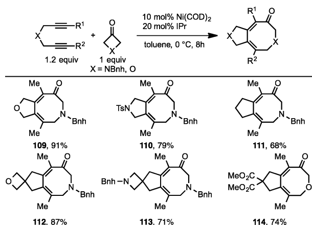
Scheme 38. Ni/P( p -tol) 3 -Catalyzed Cycloaddition of 1,3-Dienes with 3-Azetidinones and 3-Oxetanones
