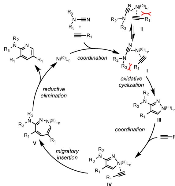
Scheme 21. Proposed Mechanism for the Ni/SIPr-Catalyzed Cycloaddition of Terminal Alkynes and Cyanamides
