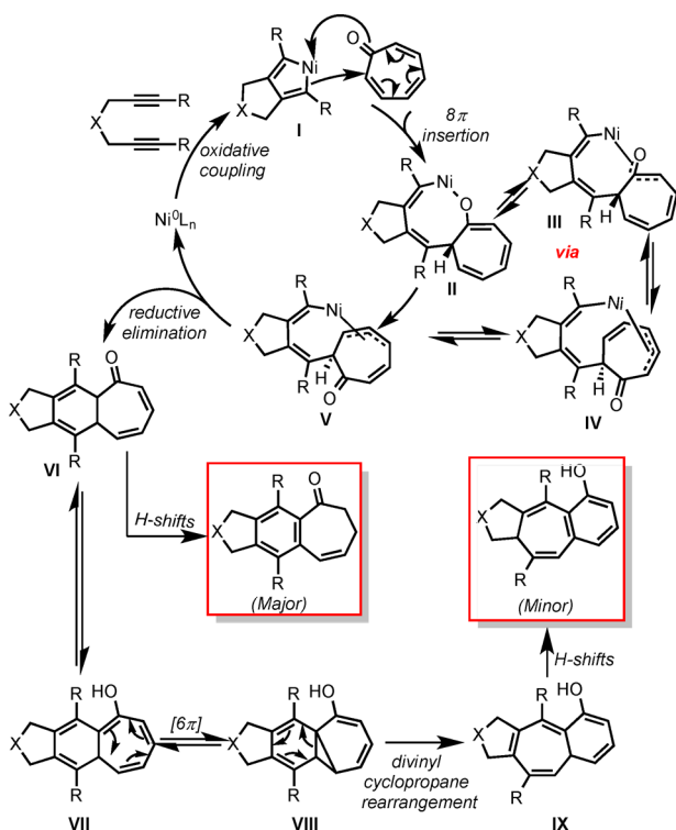
Scheme 33. Ni/PPh 3 -Catalyzed Cycloaddition of Alkynes and 3-Azetidinones
