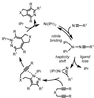
Scheme 19. Proposed Mechanism for the \text{Ni}(\text{IPr})_2 -Catalyzed Cycloaddition of Diynes and Nitriles
