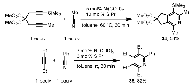
Scheme 13. Ni/SIPr-Catalyzed Cycloaddition of Unsymmetrical Diyne with Acetonitrile and 3-Hexyne with Benzonitrile
