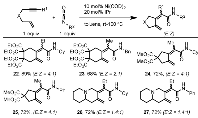
Scheme 11. Ni/IPr-Catalyzed Cycloaddition of Enynes and Isocyanates
