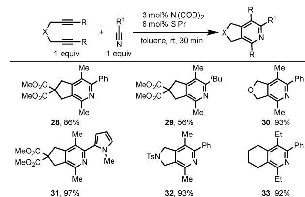
Scheme 12. Ni/SIPr-Catalyzed Cycloaddition of Diynes and Nitriles
