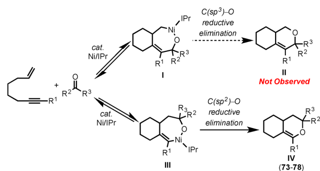
Scheme 28. Proposed Mechanism for the Ni/SIPr-Catalyzed Cycloaddition of Enynes and Ketones
