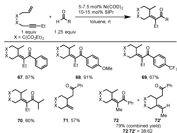
Scheme 25. Ni/SIPr-Catalyzed Cycloaddition of Enynes and Aldehydes
