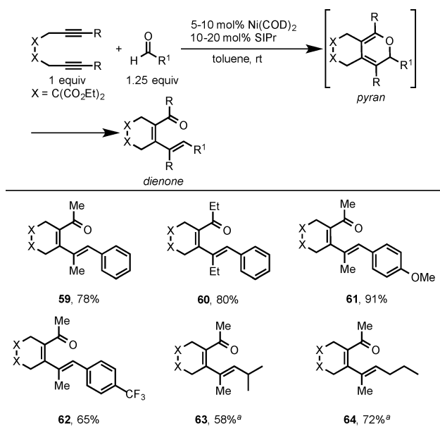
Scheme 22. Ni/SIPr-Catalyzed Cycloaddition of Diynes and Aldehydes
